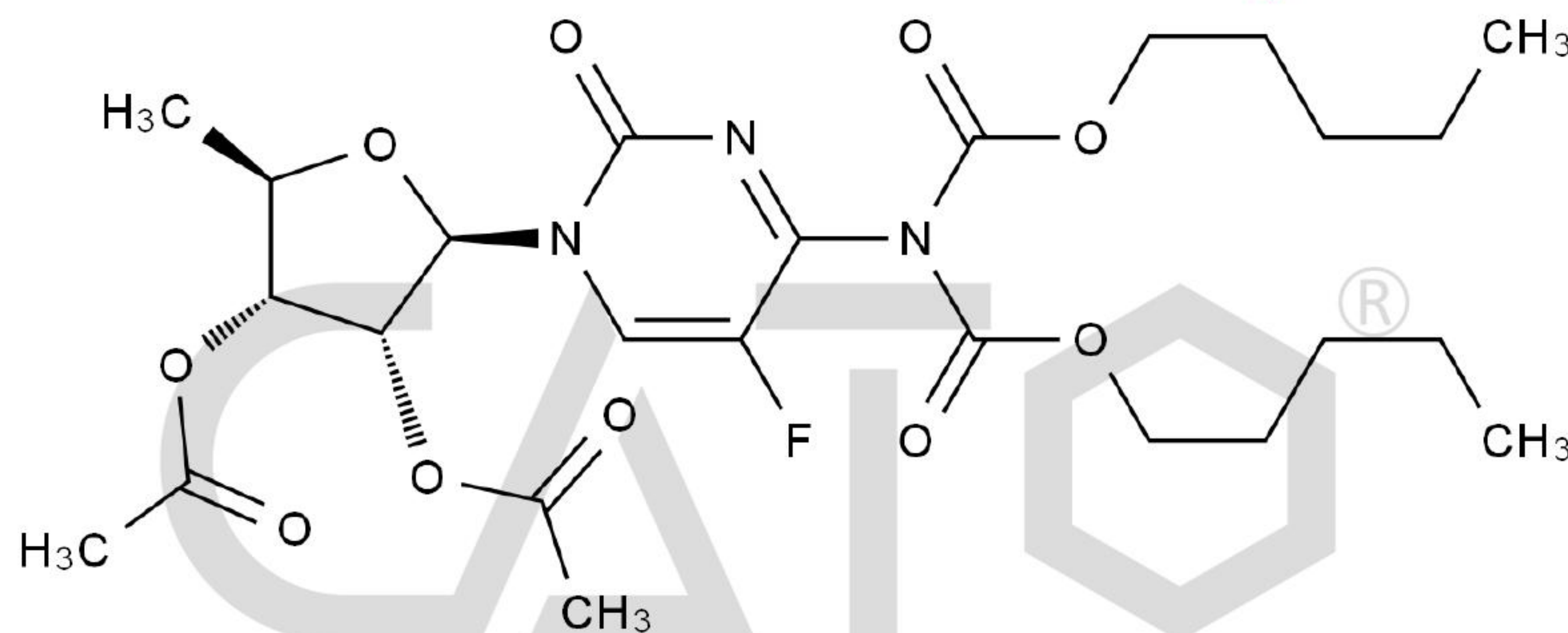
Chemical Structure:
