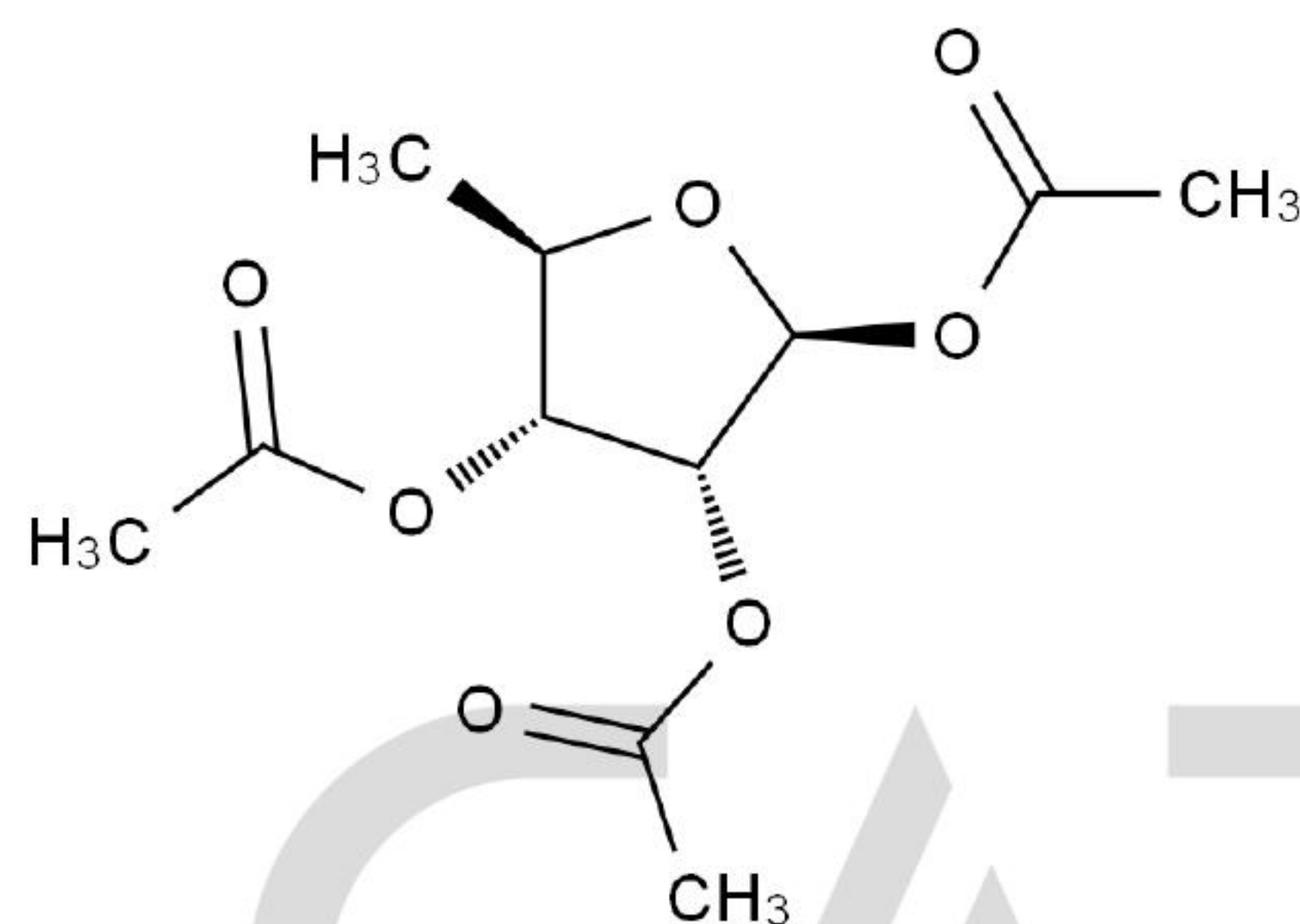
Chemical Structure:
