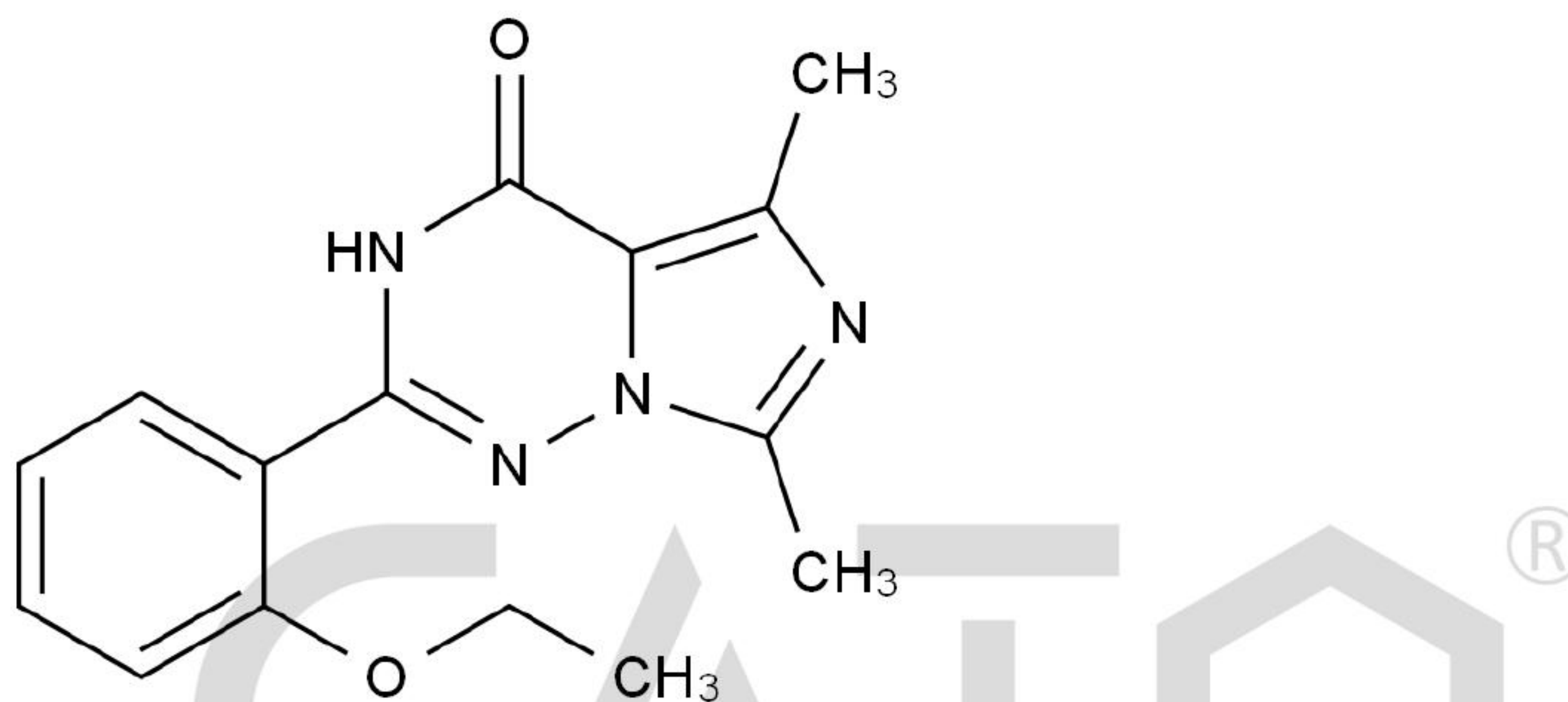
Chemical Structure:
