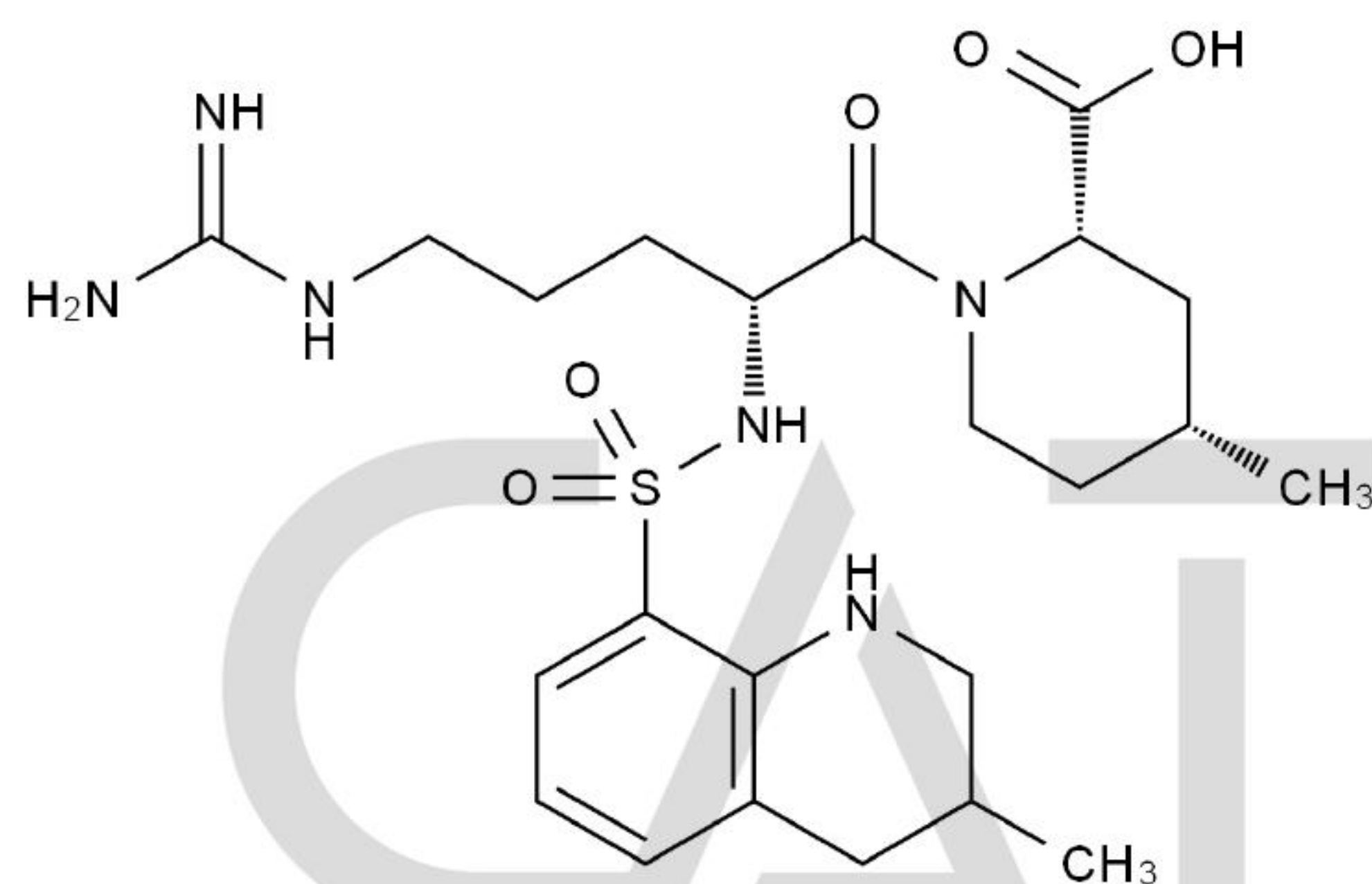
Chemical Structure:
