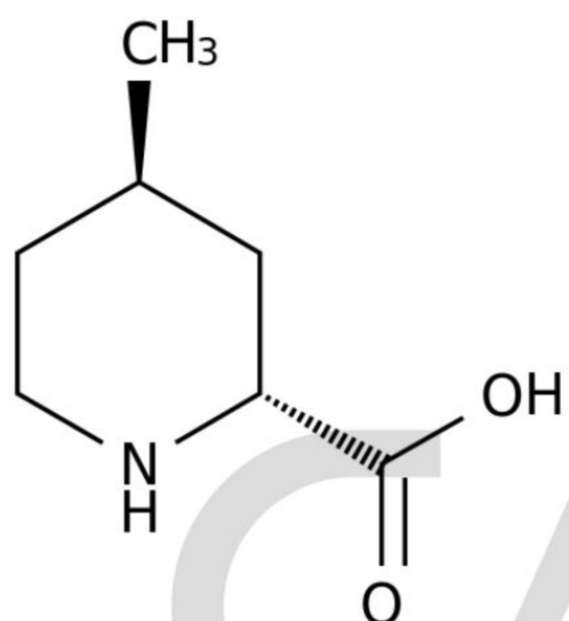
Chemical Structure:
