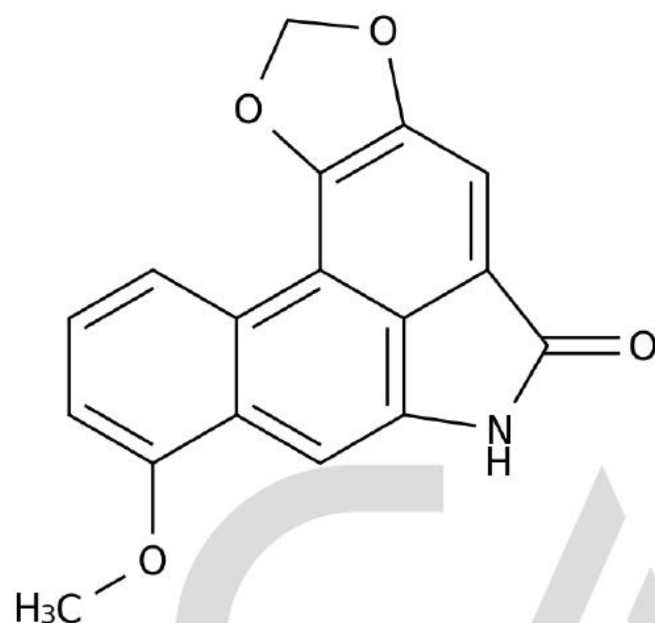
Chemical Structure:
