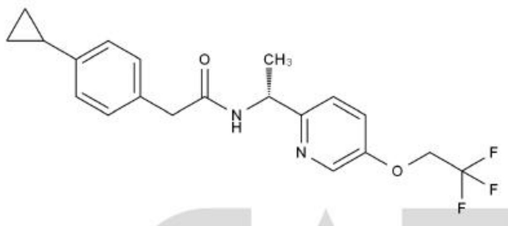
Chemical Structure:
