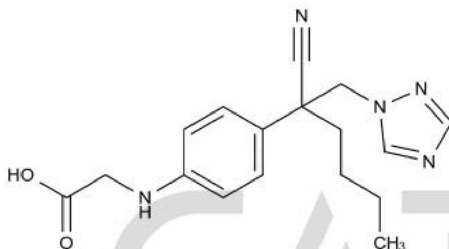
Chemical Structure:
