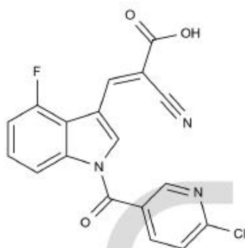
Chemical Structure:
