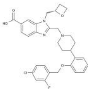
Chemical Structure:
