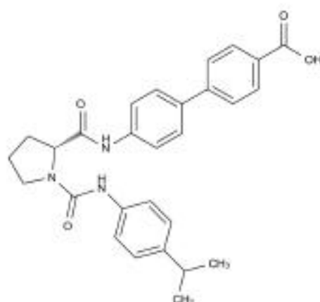
Chemical Structure:
