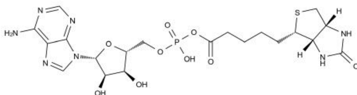
Chemical Structure:
