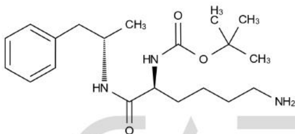
Chemical Structure:
