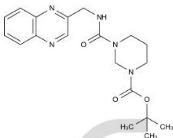
Chemical Structure:
