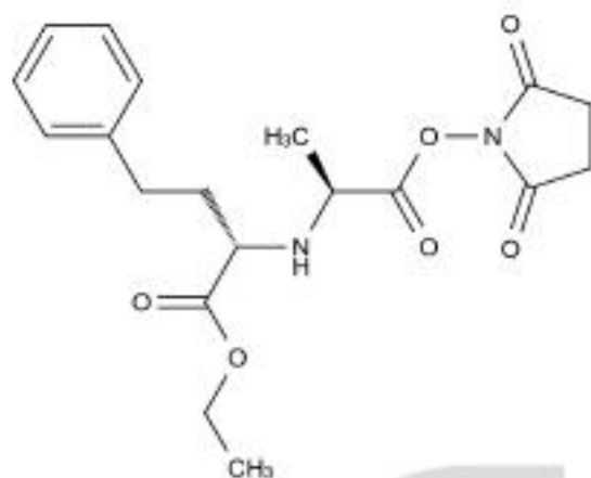
Chemical Structure:
