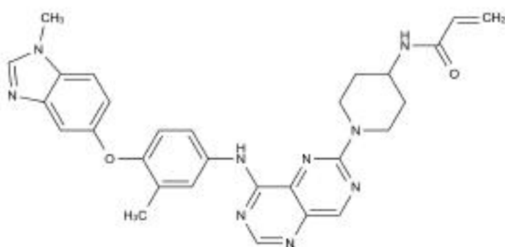
Chemical Structure:
