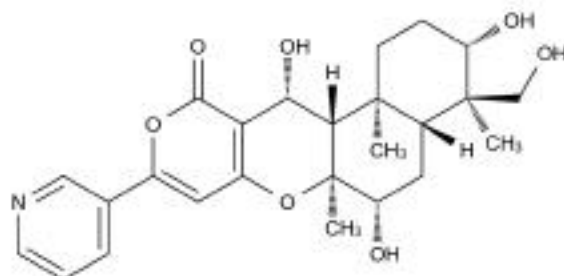
Chemical Structure:
