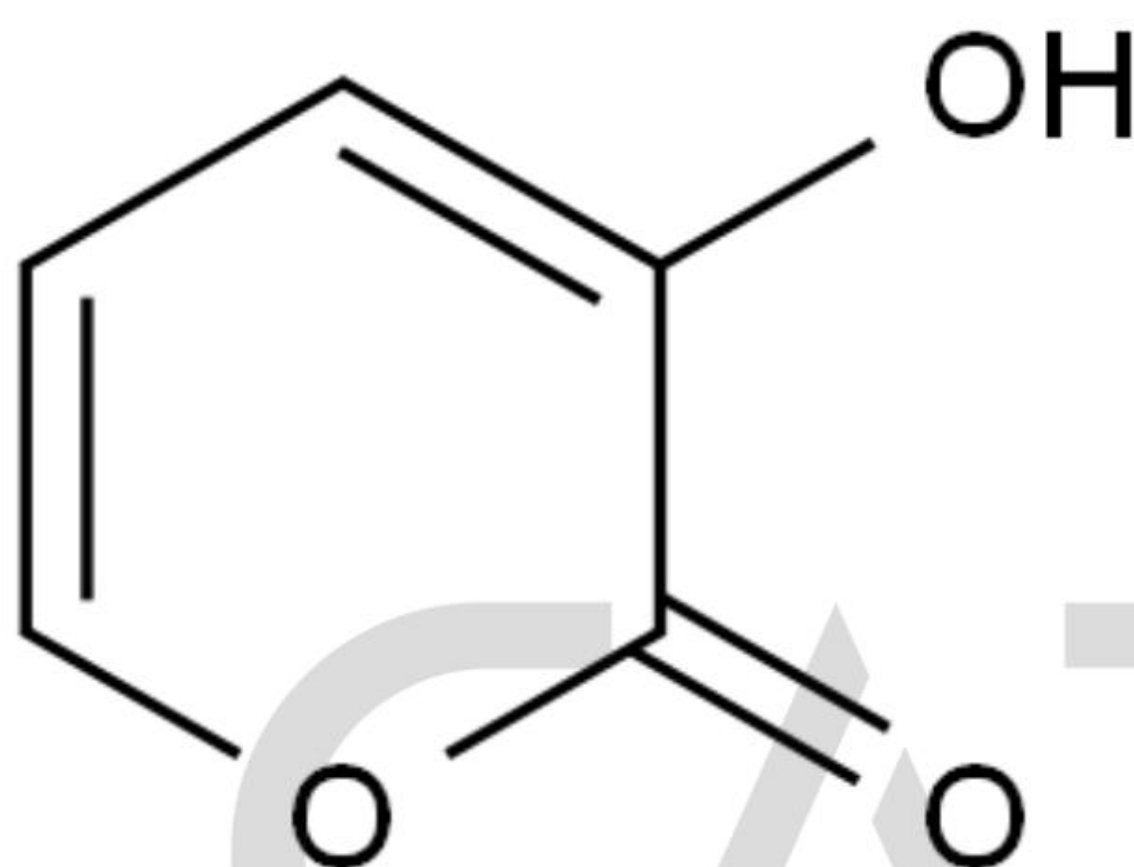
Chemical Structure:
