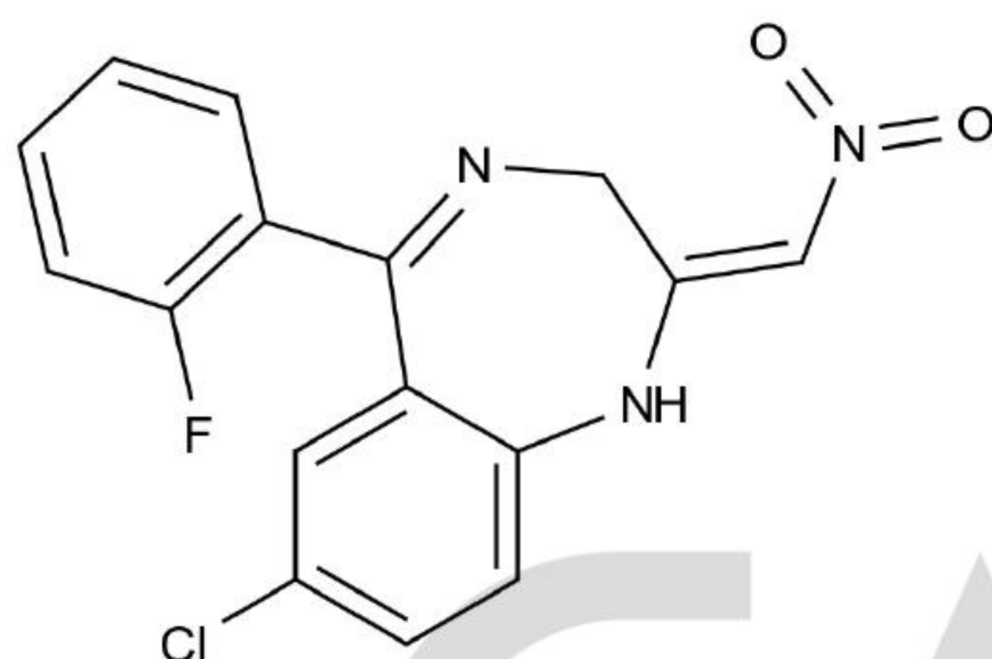
Chemical Structure:
