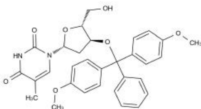
Chemical Structure:
