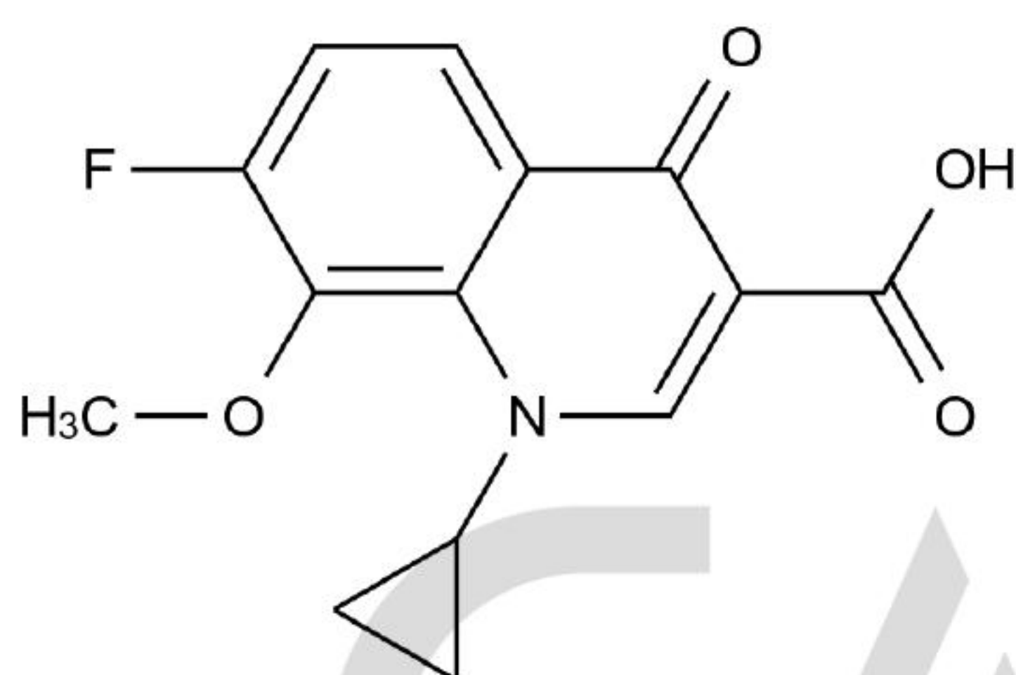
Chemical Structure:
