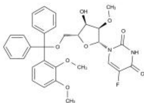
Chemical Structure:
