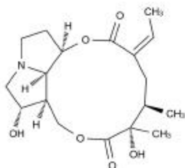
Chemical Structure:
