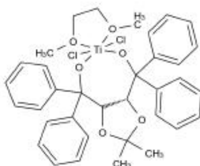
Chemical Structure:
