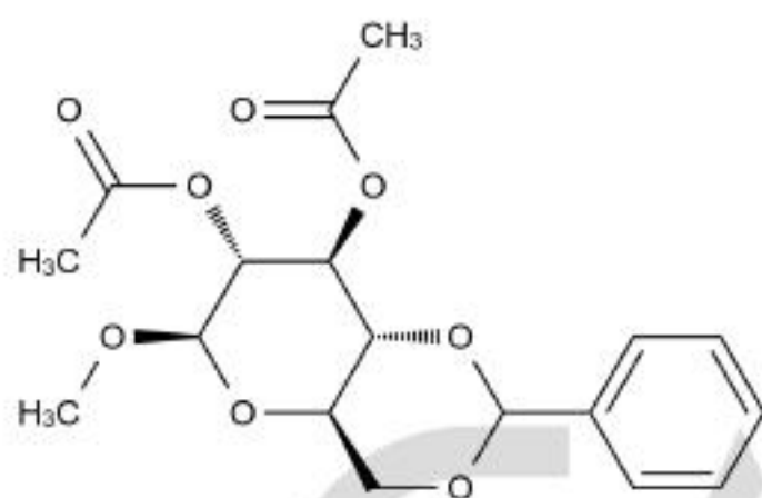
Chemical Structure:
