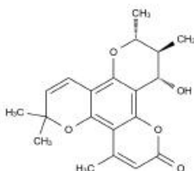
Chemical Structure:
