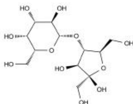
Chemical Structure:
