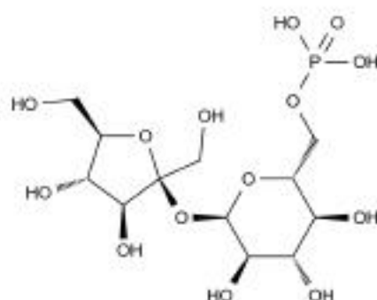
Chemical Structure:
