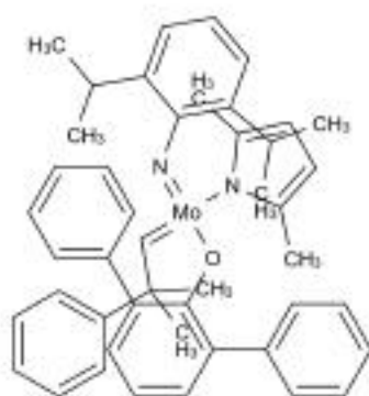
Chemical Structure:
