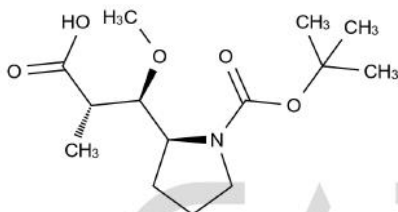
Chemical Structure:
