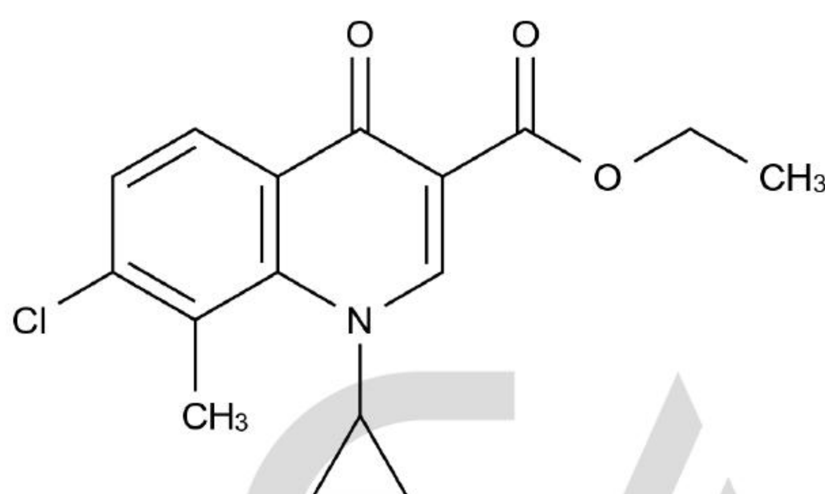
Chemical Structure:
