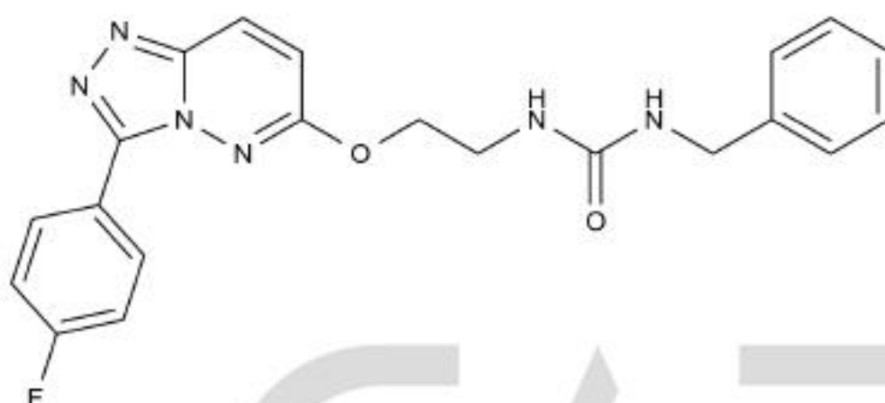
Chemical Structure:
