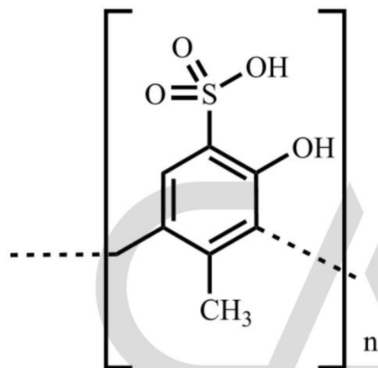
Chemical Structure:
